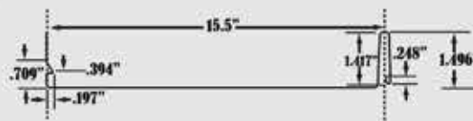
SL-LOK 1 1/2" Available in 24 Gauge and .032" Aluminum
