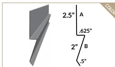
STUCCO STOP
