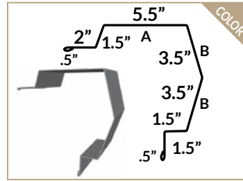
SCULPTURED RAKE
