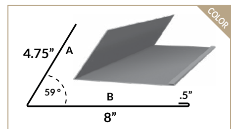
CHIMNEY FLASHING
