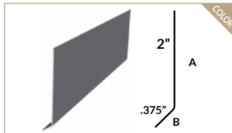
EAVE CLEAT
