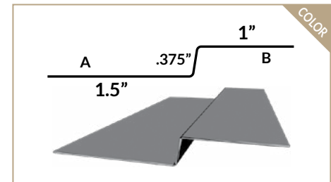
PANEL STARTER
