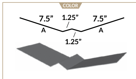
W-VALLEY
