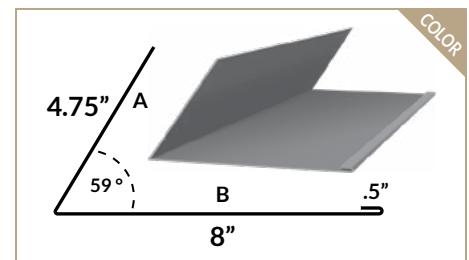
CHIMNEY FLASHING
