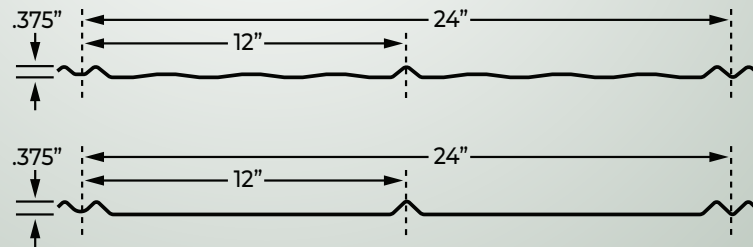
Overlap Details
