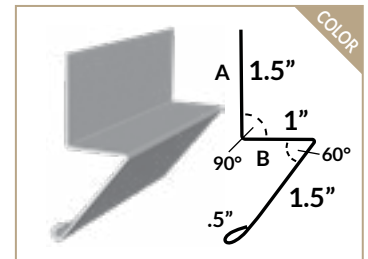
BASE ANGLE
