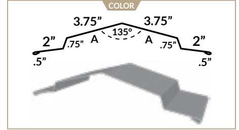
RIDGE CAP
