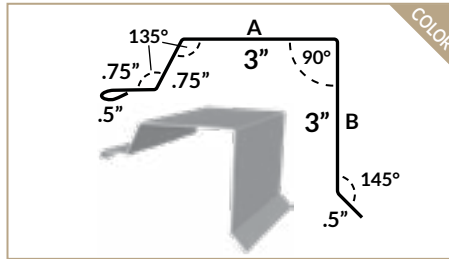
5V GABLE
