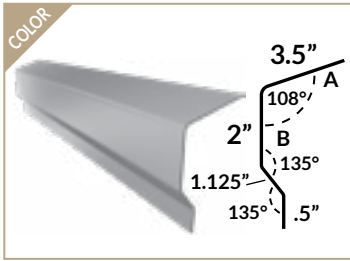
DRIP COVER
