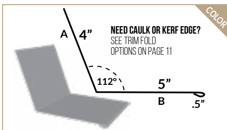
FLAT ENDWALL
