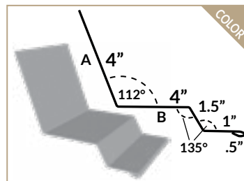
PBR ENDWALL
