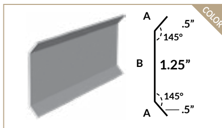
COUNTER FLASHING
