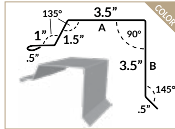
PBR GABLE
