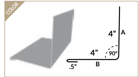
SIDEWALL
