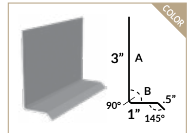
DRIP CAP
