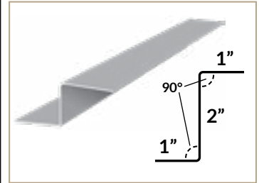
Z FLASHING 2"
