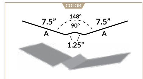
W-VALLEY
