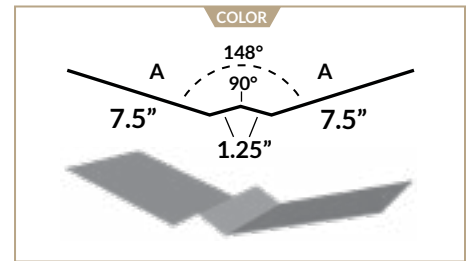
W-VALLEY
