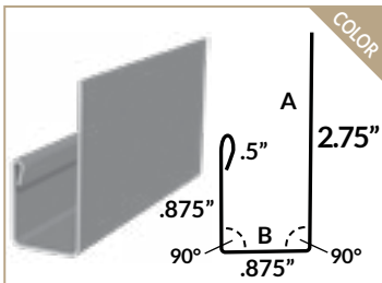
J CHANNEL
