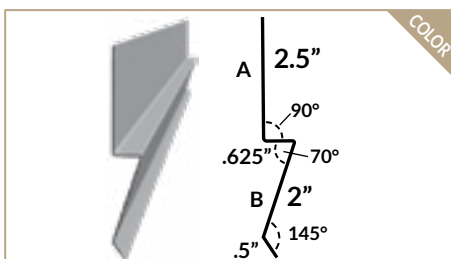
STUCCO STOP
