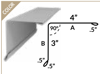
GABLE 1"
