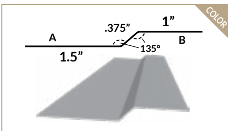
PANEL STARTER
