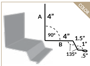
PBR SIDEWALL
