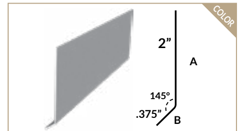
EAVE CLEAT
