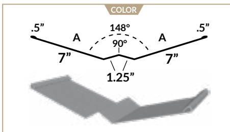
HEMMED W-VALLEY
