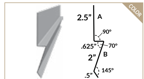
STUCCO STOP
