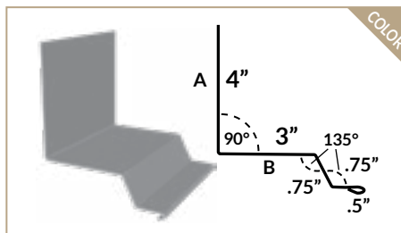
5V SIDEWALL
