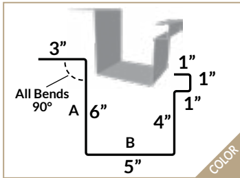
BOX GUTTER
