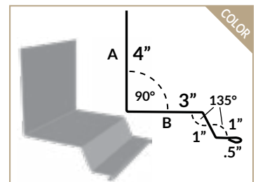
SIDEWALL
