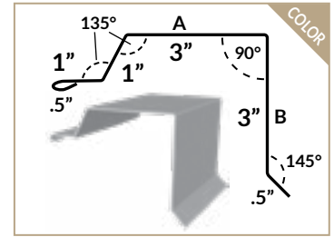
GABLE
