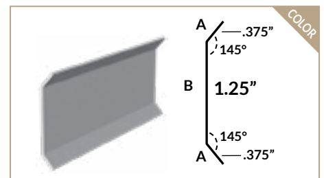
COUNTER FLASHING
